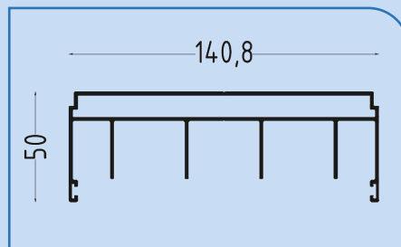
ΑΝΩ ΟΔΗΓΟΣ / UPPER RAIL - 4RAIL
