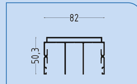
ΑΝΩ ΟΔΗΓΟΣ / UPPER RAIL - 3RAIL
