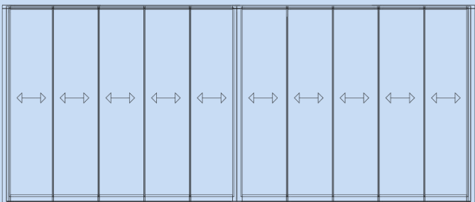
5 RAIL SINGLE GLASS SLIDING 5+5 PANELS
