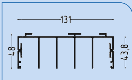
ΑΝΩ ΟΔΗΓΟΣ / UPPER RAIL - 5RAIL
